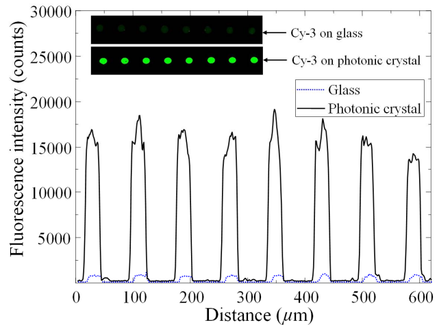
Fig. 5. Intensity profile as a function of distance for a line of fluorescent image pixels profiling spots of Cy-3 conjugated streptavidin for both the glass slide and the PC under normal incidence illumination. The scanned images are shown in insets.
