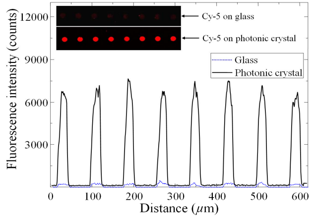
Fig. 4. Intensity profile as a function of distance for a line of fluorescent image pixels profiling spots of Cy-5 conjugated streptavidin for both the glass slide and the PC under normal incidence illumination. The scanned images are shown in insets.
