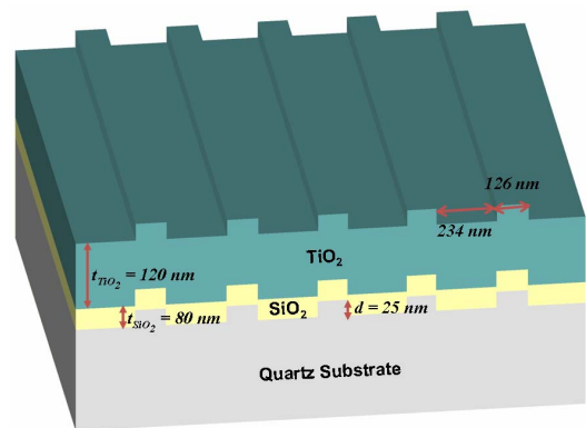
Fig. 1. Cross-sectional diagram (not to scale) of the PC. The dimensions are as follows: d = 360 nm, grating depth d = 25 nm, SiO 2 thickness t_{\text{SiO}_2} = 80 nm and TiO 2 thickness t_{\text{TiO}_2} = 120 nm. The grating width is 35% of the period.
