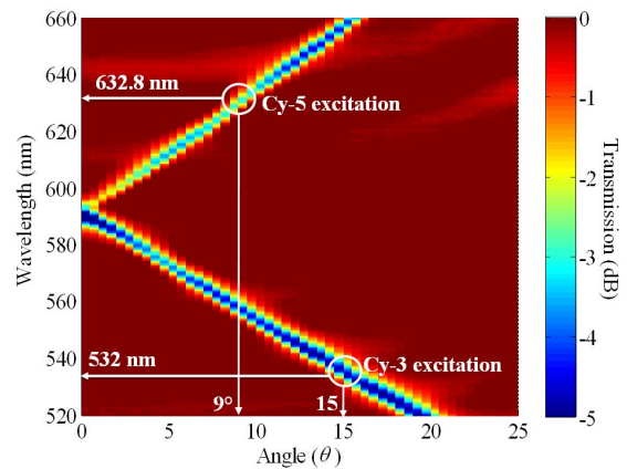
Fig. 3. Measured dispersion diagram for the PC used in this study by RCWA. Resonance for the enhanced excitation for the TM mode is \theta \sim 9^\circ for Cy-5 excitation and \theta \sim 15^\circ for Cy-3 excitation.
