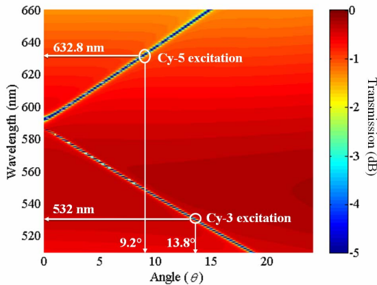
Fig. 2. Simulated dispersion diagram for the PC used in this study by RCWA. Resonance for the enhanced excitation for the TM mode is \theta \sim 9.2^\circ for Cy-5 excitation and \theta \sim 13.8^\circ for Cy-3 excitation.
