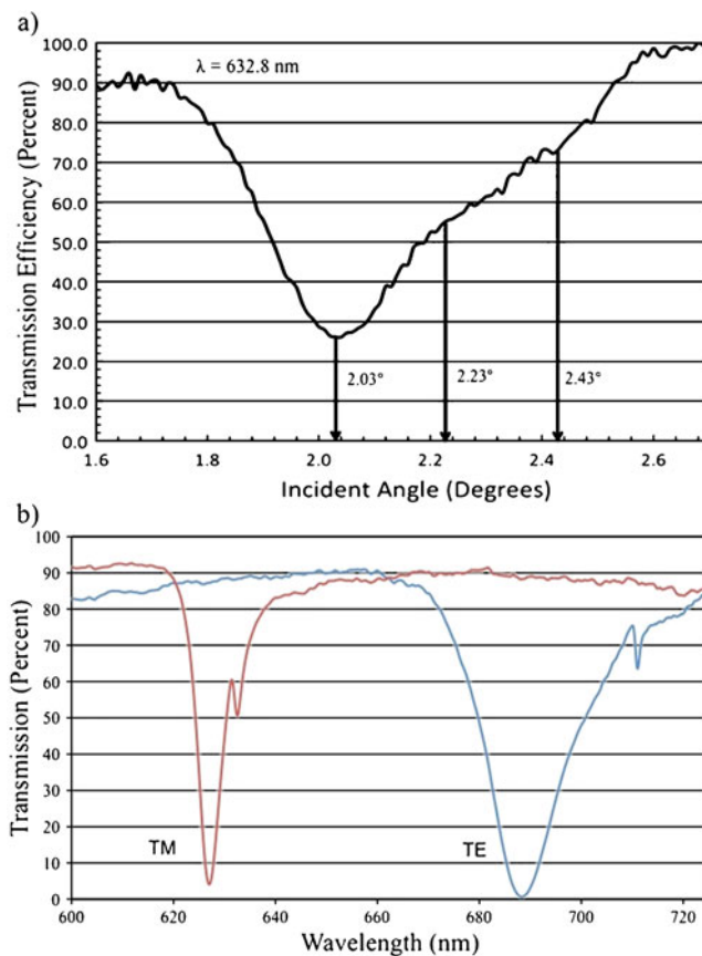
Fig. 3 Angular transmission spectrum for the TM enhanced excitation mode showing the choice of various angles of excitation a to generate optimal on-resonance excitation at an incident angle of 2.03^\circ . Transmission efficiency versus wavelength b showing dips in transmission intensity at normal incidence for the TE ( \lambda=690 nm) and TM ( \lambda=625 nm) modes. Wavelengths of maximum resonance reflection correspond to wavelengths of minimum transmission
