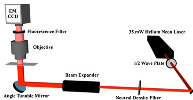
Fig. 2 Detection instrument used for photonic crystal enhanced fluorescence photobleaching study. A HeNe laser beam is expanded and collimated before reflection from an angle-tunable mirror that illuminates the photonic crystal device from below. The fluorescence emission is gathered by a conventional microscope objective and measured using a cooled EM-CCD camera
