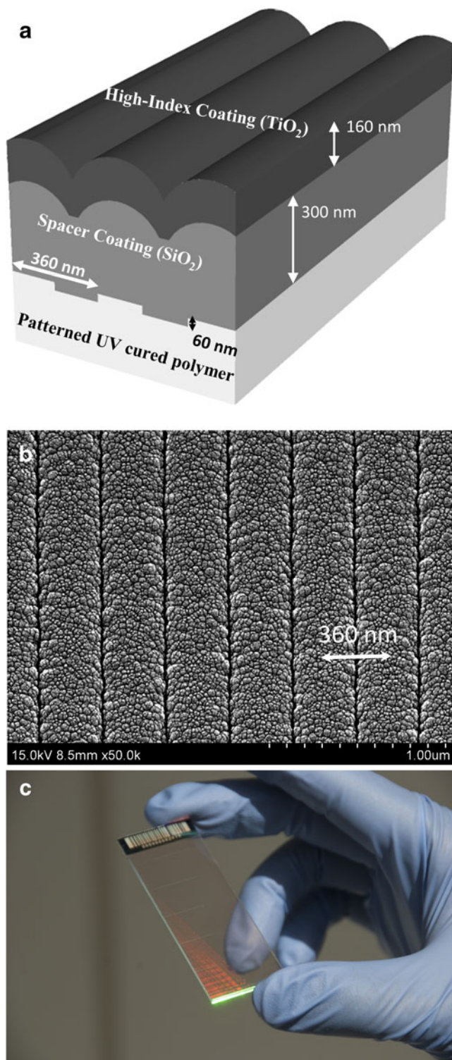
Fig. 1 Schematic cross section diagram of the photonic crystal structure (a), with a top view electron microscope image (b), and a photograph of the device attached to a standard glass microscope slide (c)
