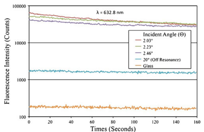
Fig. 5 Plot of the measured fluorescence intensity versus time for continuous exposure at different angles of incidence for the excitation light
