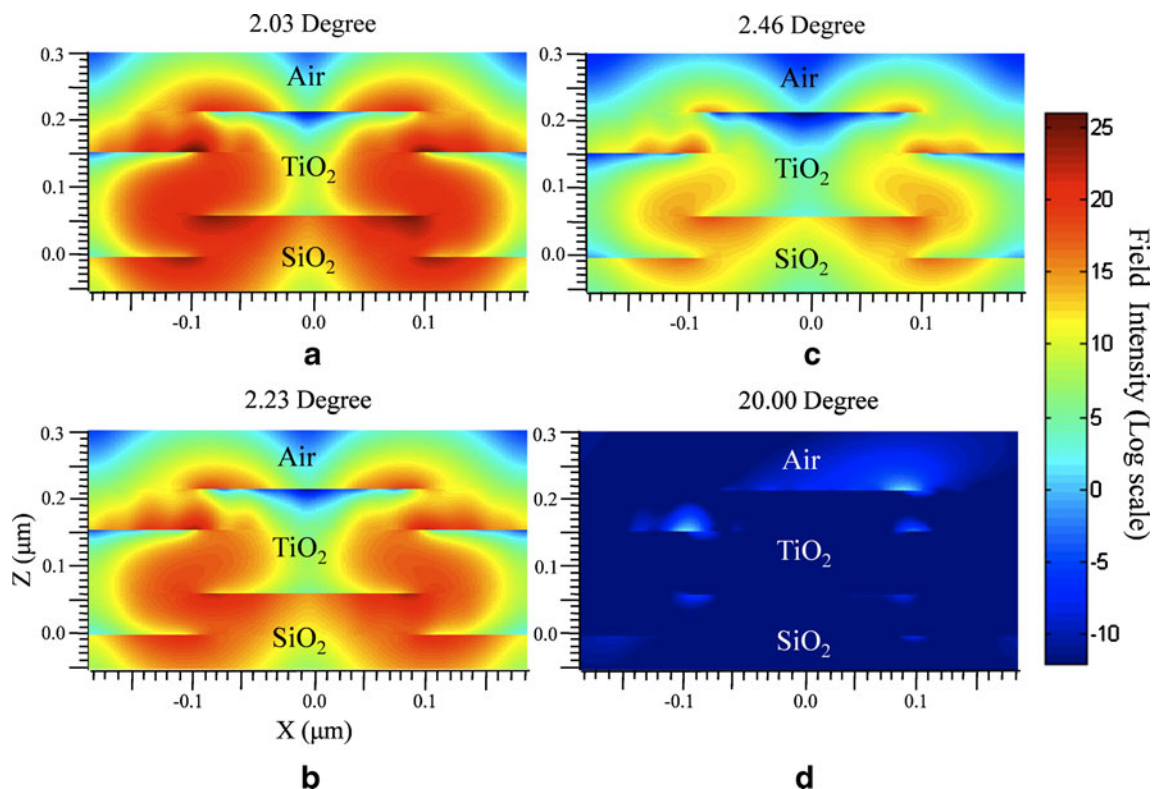
Fig. 6 Electric field intensity plots generated using rigorous coupled wave analysis for excitation conditions corresponding to 2.03° (a), 2.23° (b), 2.46° (c) and 20° (d). The electric field in the medium
