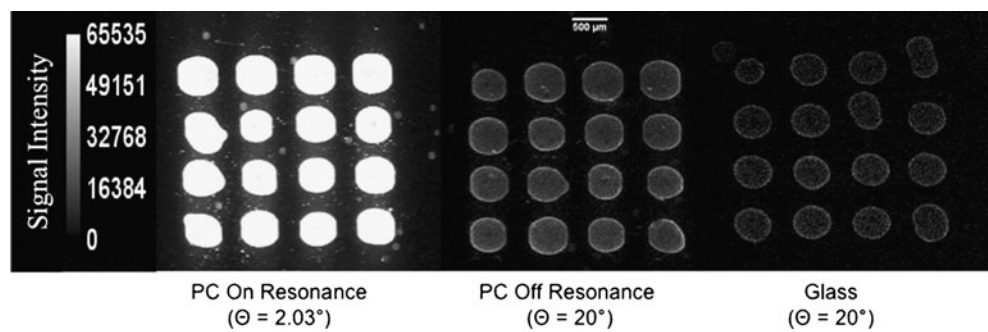
Fig. 4 Images of Cy5-streptavidin spots taken for photonic crystal on-resonance ( left ), photonic crystal off-resonance ( middle ) and an unpatterned glass slide ( right ). Images were gathered with equal exposure and camera settings for direct comparison
